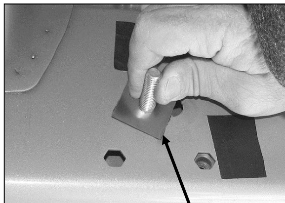
12mm x 40mm Bolt x 10mm Nut Plate w/ 12mm Plastic Retainer
