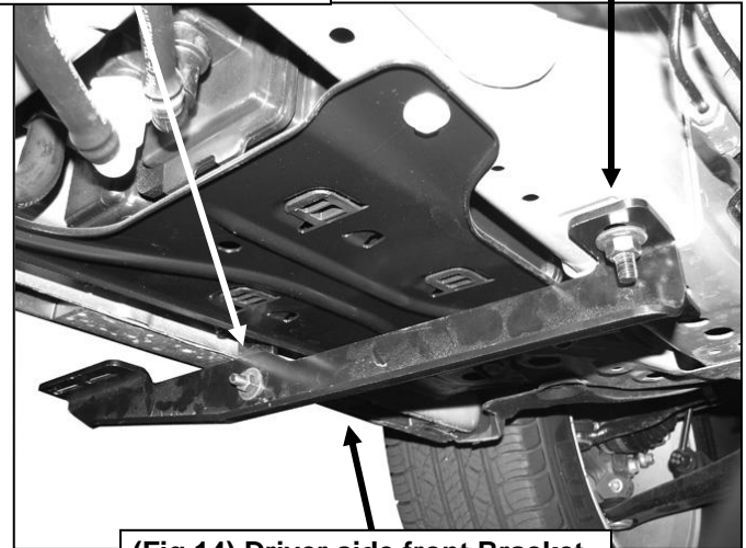
(Fig 14) Driver side front Bracket pictured installed without cover for instructions purposes only
