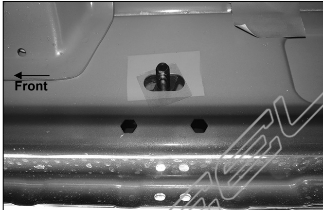
(Fig 6) Passenger/right center mounting location (2013-on pictured with factory holes)
