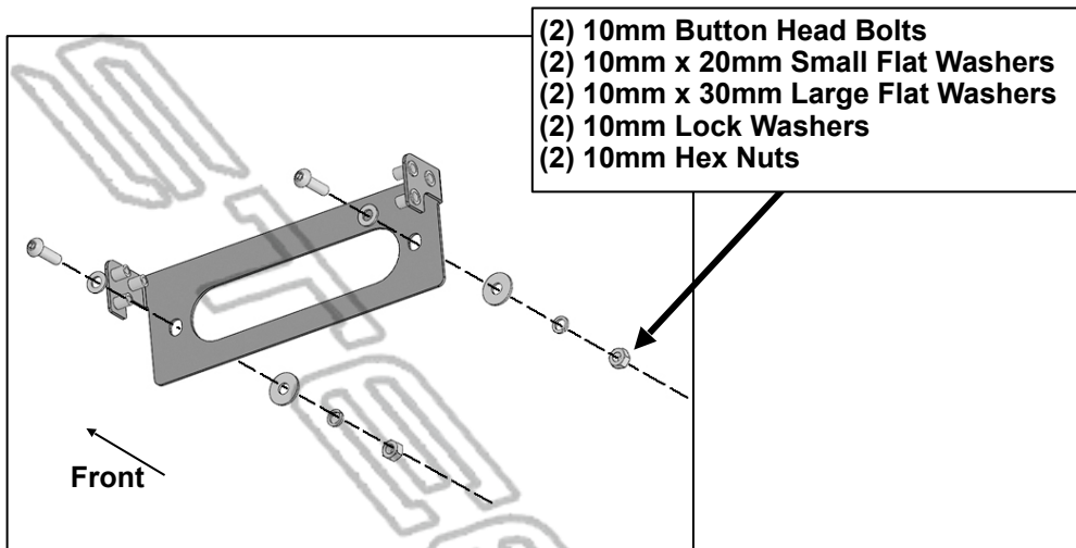
(Fig 1) Attach the Mounting Bracket to the winch opening on the front of the bumper
