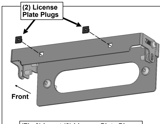
(Fig 3) Insert (2) License Plate Plugs into the License Plate Bracket
