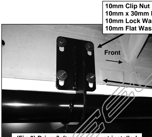
(Fig 6) Driver/left center mount installed
