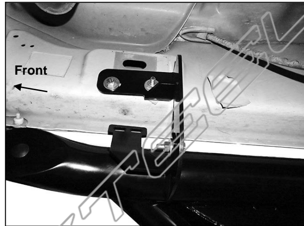
(Fig 12) 2009-10 passenger/right front pictured
