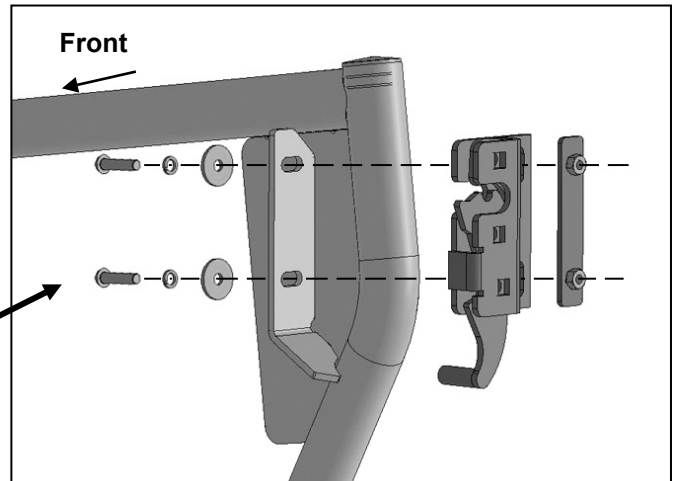
(Fig 6) Attach passenger/right Door Latch to Door
