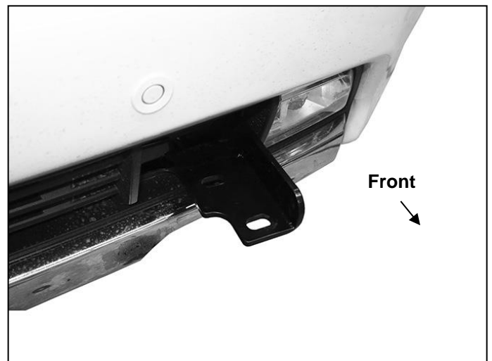
(Fig 13) Driver/left Frame Bracket installed
