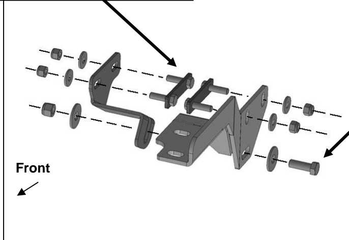
(Fig 8) Models without tow hooks, insert the included (2) 10mm Double Bolt Plates into the open end of the frame and out the holes in the sides. Attach the Driver/left outer Frame Bracket and inner Support Bracket to the sides of the frame and Bolt Plates
