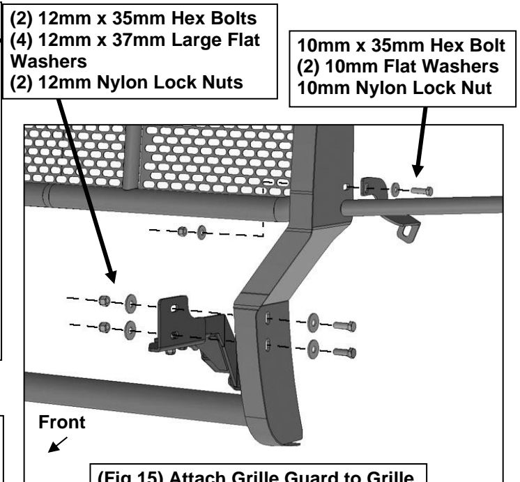
(Fig 15) Attach Grille Guard to Grille Guard Bracket and Top Bracket
