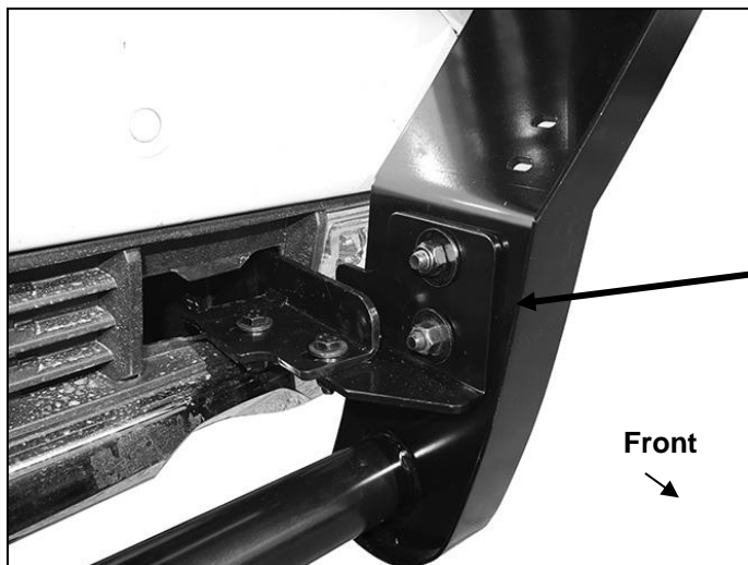
(Fig 16) Attach Grille Guard to Frame Bracket
