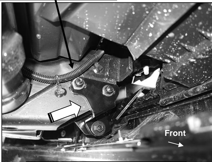
(Fig 12) Attach Driver/left inner Support Bracket to Frame Bracket and Double Bolt Plate in frame (arrow)
