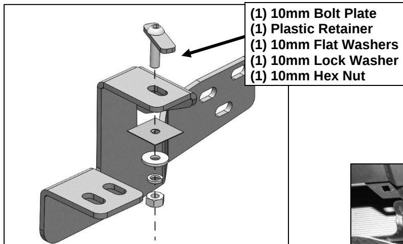
(Fig 5) Attach Frame Mounting Bracket
