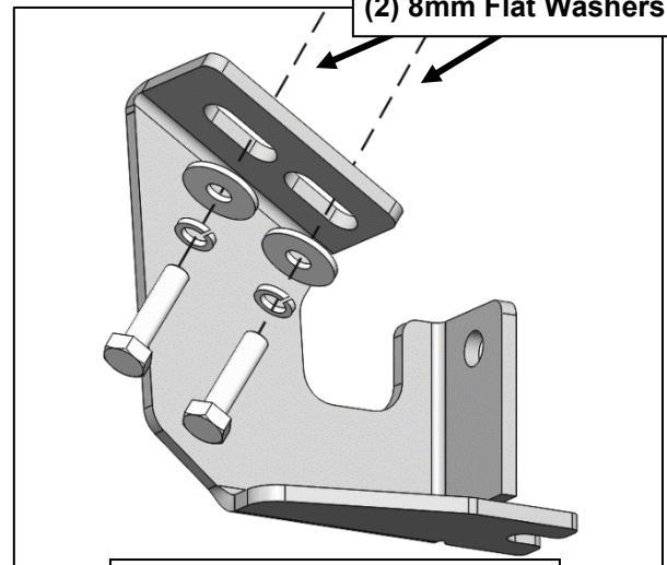
(Fig 11) Passenger/Right Center/Rear Mounting Bracket
