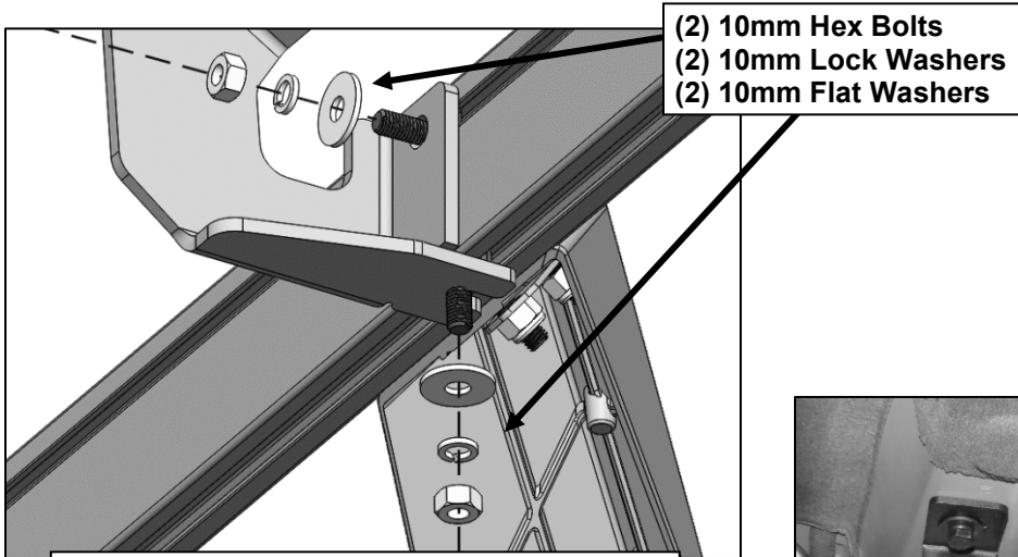
(Fig 13) Attach Passenger/Right Main Tube to all Passenger/Right Mounting Brackets
