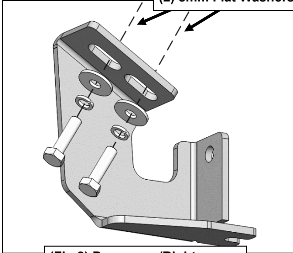
(Fig 8) Passenger/Right Center/Rear Mounting Bracket
