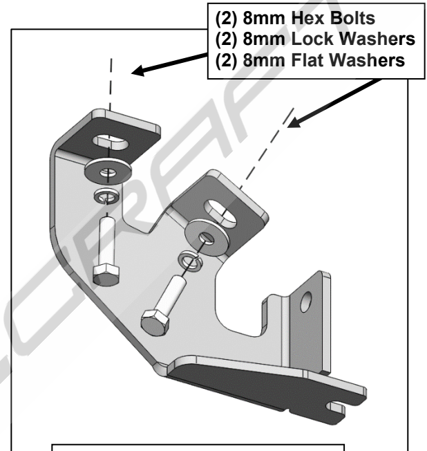
(Fig 5) Attach Passenger/Right Front Mounting Bracket
