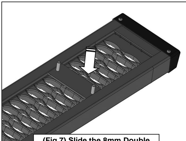
(Fig 7) Slide the 8mm Double Bolt Plate into channels
