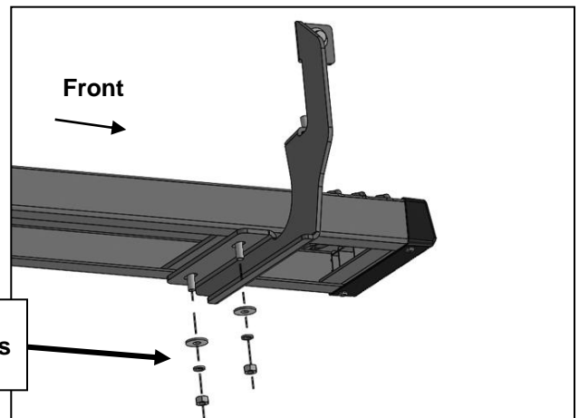
(Fig 8) Running Board attached to Driver/left side front Mounting Bracket
