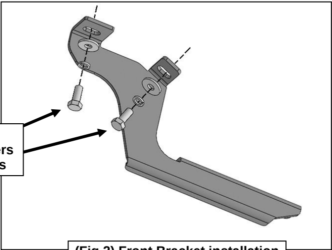
(Fig 2) Front Bracket installation
