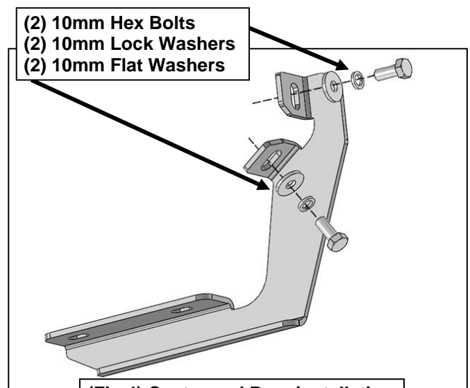
(Fig 4) Center and Rear installation
