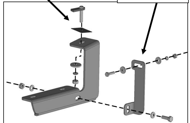
(Fig 16) Passenger/right #2, #3 and rear Brackets illustrated
