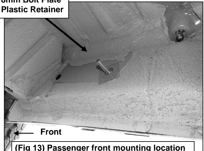
(Fig 13) Passenger front mounting location
