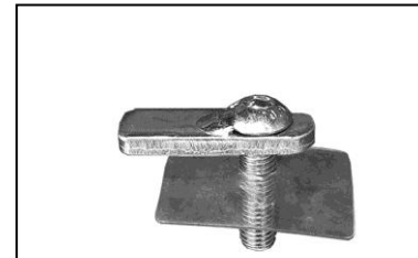
(Fig 2) 8mm Bolt Plate with Plastic Retainer
