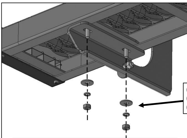
(Fig 10) Attach Running Board to Brackets
