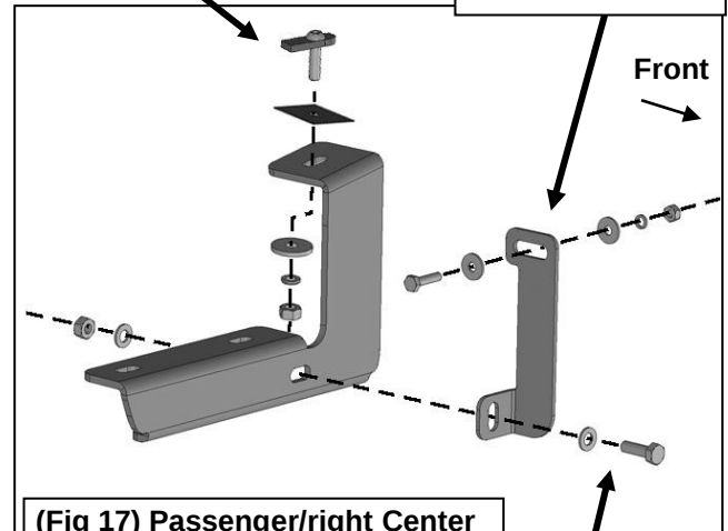
(Fig 17) Passenger/right Center and rear Brackets illustrated
