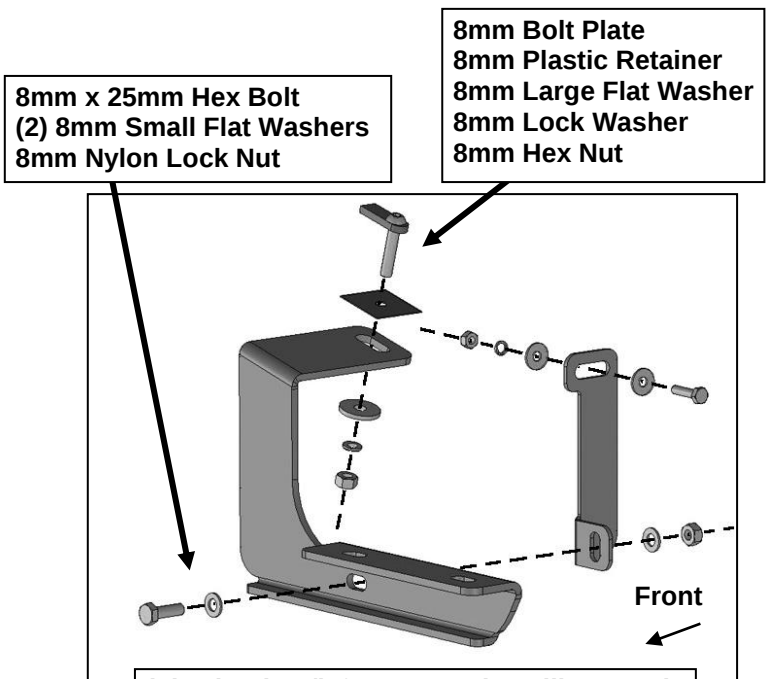
(Fig 7) Driver/left rear Brackets illustrated
