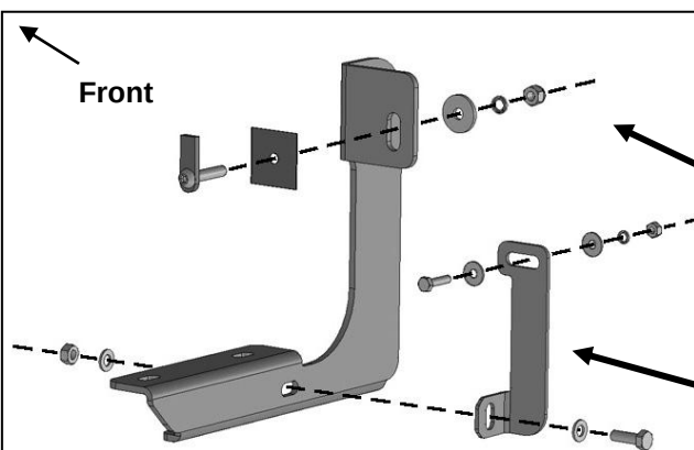
(Fig 15) Passenger/right front Mounting Bracket and Support Bracket illustrated
