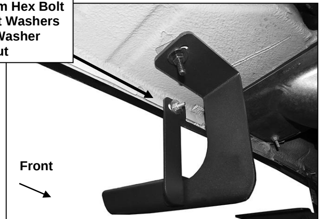
(Fig 12) Mark and drill hole through pinch weld. Attach top of Driver/left rear Support Bracket to back of pinch weld. Reinstall Running Board
