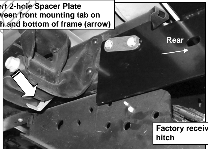
(Fig 8) Driver side installation with hitch
