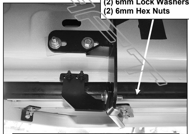
(Fig 20B) Driver/left rear Bracket assembly (Example of Mega Cab installation)
