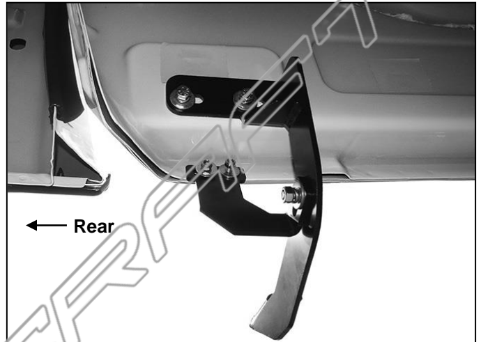
(Fig 16) Driver/Left rear Mounting Bracket assembly
