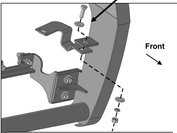
(Fig 18) driver side 2013-18 Upper Bracket
