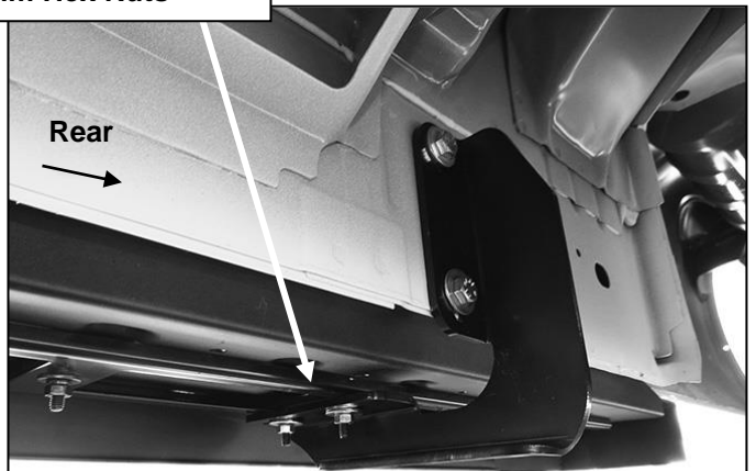
(Fig 11) Passenger/right rear Bracket installed
