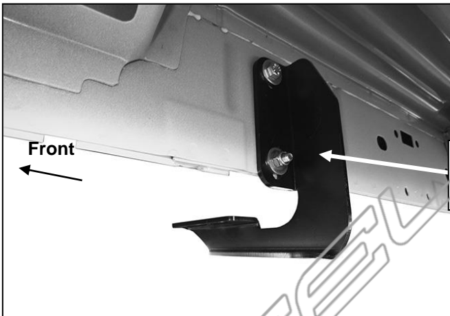
(Fig 5) Passenger/right center Bracket installed
