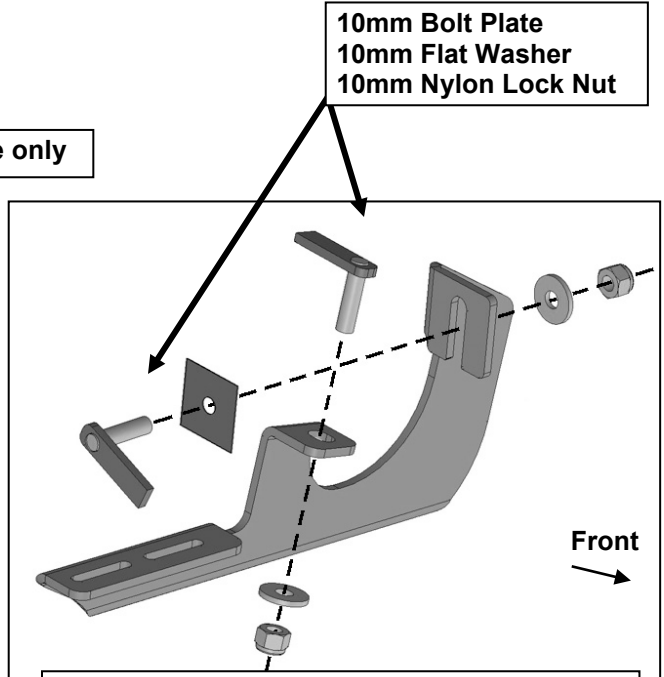
(Fig 10) Passenger side #3 Mounting Bracket
