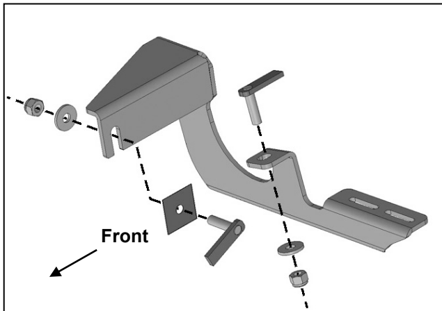
(Fig 23) Driver side front Mounting Bracket
