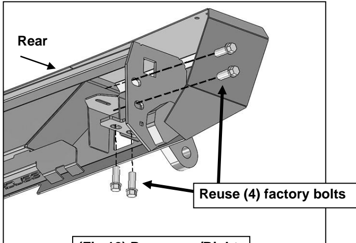
(Fig 12) Passenger/Right side of Bumper installed
