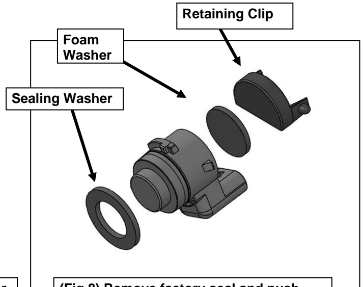
(Fig 8) Remove factory seal and push Flat Sealing Washer onto end of sensor
