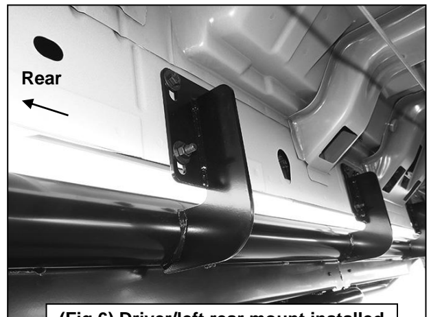
(Fig 6) Driver/left rear mount installed
