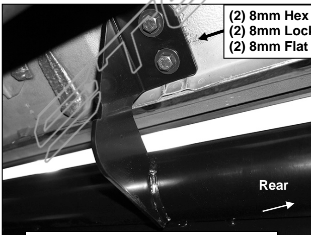
(Fig 5) Passenger side rear installed
