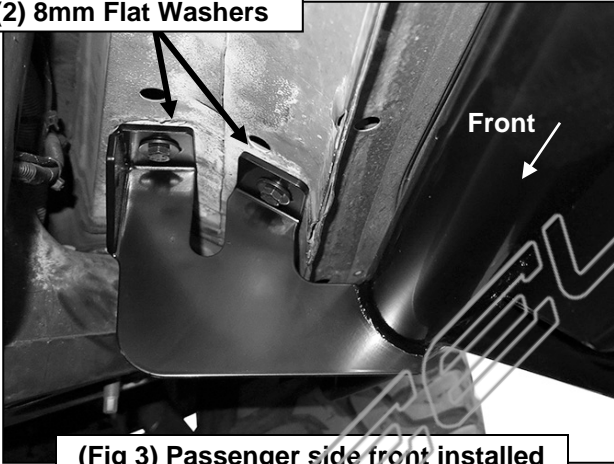
(Fig 3) Passenger side front installed
