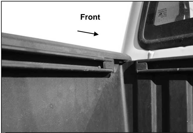
(Fig 1) Remove factory hardware attached to the ends of the bed channel (Driver side pictured)
