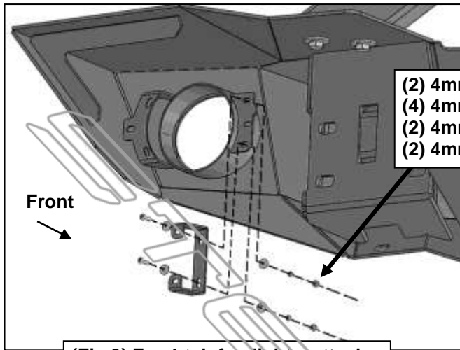
(Fig 9) For 4-tab fog lights, attach (1) U-Bracket to the mounting plate
