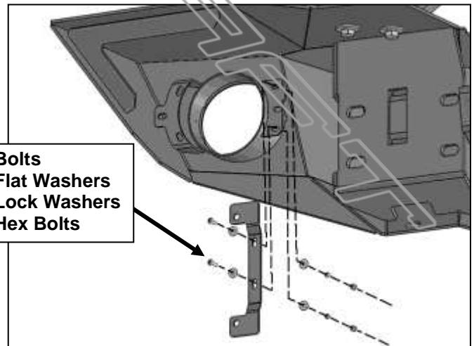
(Fig 8) LED Fog Lights, attach the Driver/Left LED Light Bracket to the mounting plate
