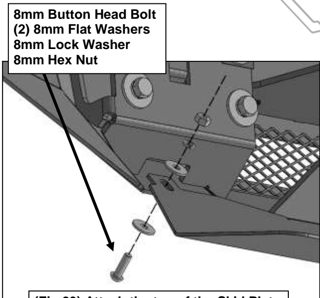
(Fig 23) Attach the top of the Skid Plate to the lower rear of the Bumper, (Driver/Left side shown)
