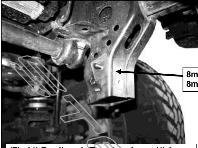
(Fig 21) For JL and JT models, insert (1) 8mm Bolt Nut Plate into the bottom of the frame and out the hole shown. (Thread (2) 12mm Plastic Retainers to hold the Bolt/Nut Plates in place)
