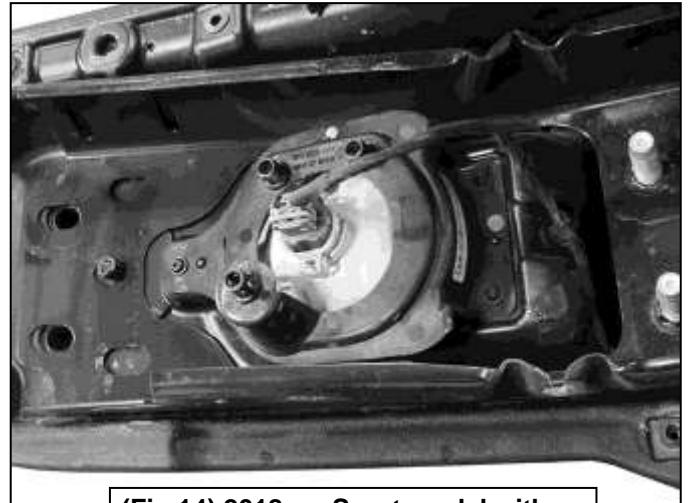
(Fig 14) 2018-on Sport model with 1pc plastic bumper cover. Driver/left Fog light assembly pictured
