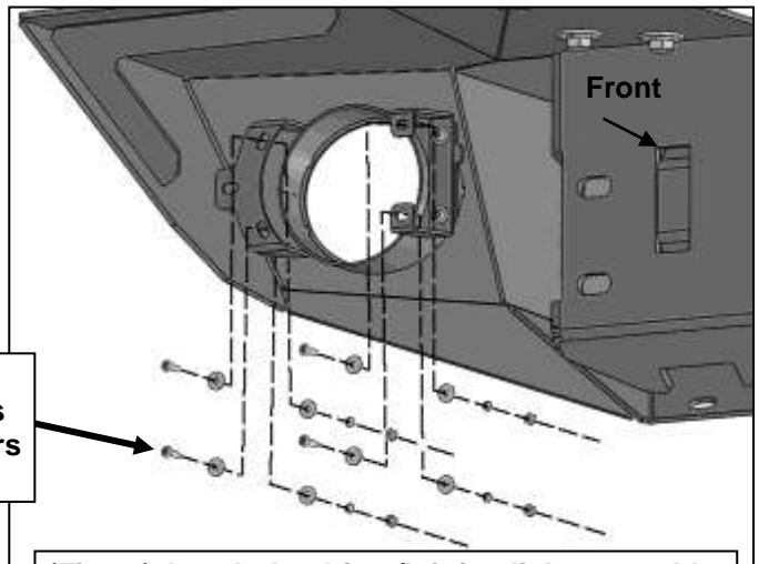
(Fig 10) Attach the driver/left fog light assembly to the Adapter Bracket and mounting plate
