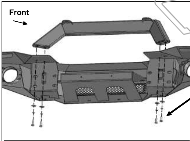
(Fig 7) Attach Bull Nose Hoop to top of Bumper
