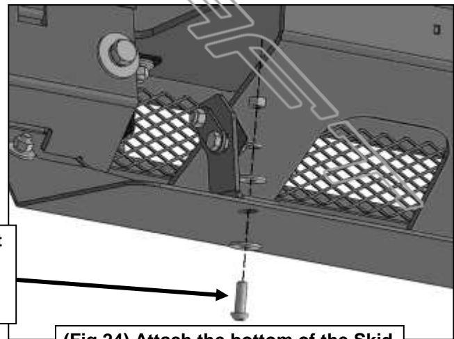
(Fig 24) Attach the bottom of the Skid Plate to the Skid Plate Brackets, (JL/JT model installation shown)
