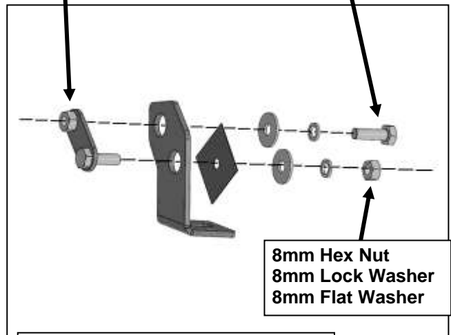
(Fig 22) For JL and JT models, attach the Driver/Left Skid Plate Bracket to the 8mm Bolt/Nut Plate
