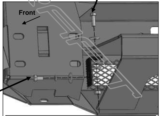
(Fig 16) Attach light bar (not included) with Brackets to mounting tabs on back of Bumper
