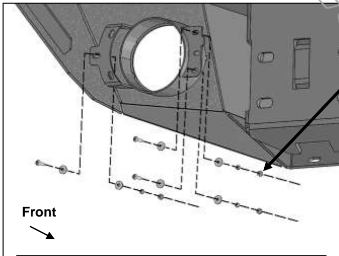
(Fig 15) Attach 2018-on Sport model fog light assembly to mounting plates, no adapters required. Driver/left side of Bumper illustrated
