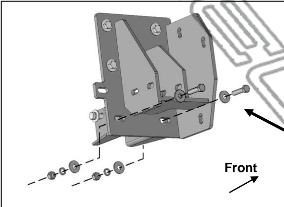
(Fig 10) Attach the Support Brackets to the bottom slots in the driver/left Frame Bracket
