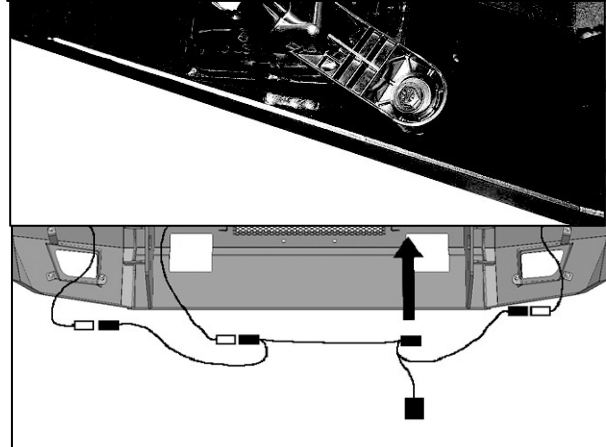
(Fig 30) Reinstall factory wiring harness over Bumper Brackets on back of Bumper. NOTE: Use the included (3) Wire Harness Extensions as necessary to reach the parking sensors
