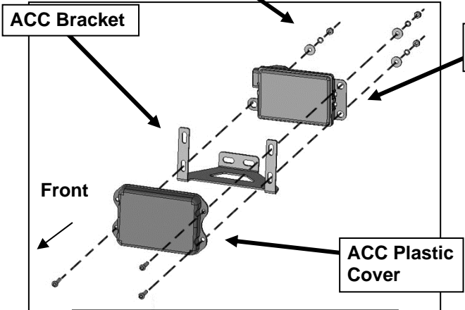
(Fig 20) Attach "Early" ACC and plastic cover to the ACC Bracket
