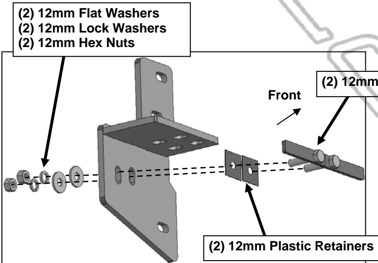
(Fig 7) Attach passenger/right side Mounting Bracket to the inner side of frame
