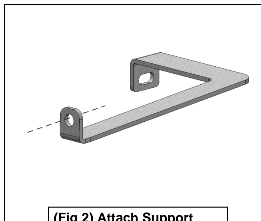
(Fig 2) Attach Support Bracket reusing hardware
