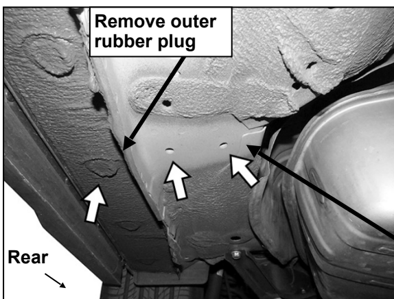
(Fig 7) Passenger/right rear mounting location. Remove outer rubber plug (arrows)
