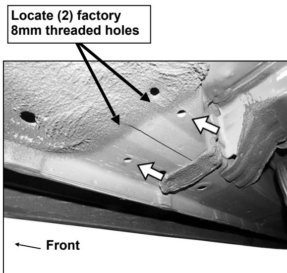
(Fig 1) Passenger/right front mounting location (arrows)
