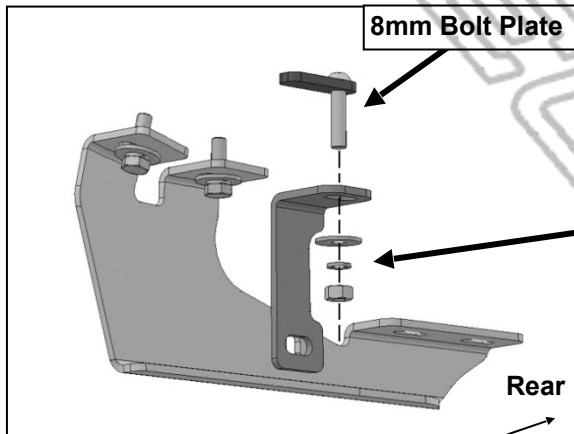
(Fig 10) Attach passenger/right rear Support Bracket to Bolt Plate
